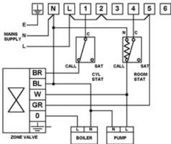
Gravity Hot water with Pumped Heating via RoomStat, CylinderStat and Two Port Zone Valve (with Changeover Auxiliary Switch) on Hot Water circuit
