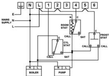
Gravity Hot water with Pumped Heating via RoomStat and CylinderStat including Frost protection via double pole FrostStat
